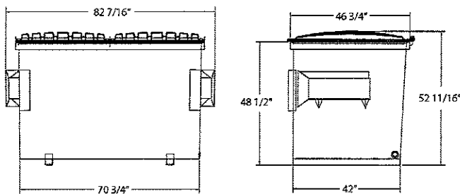
3 YARD FLAT NESTABLE
